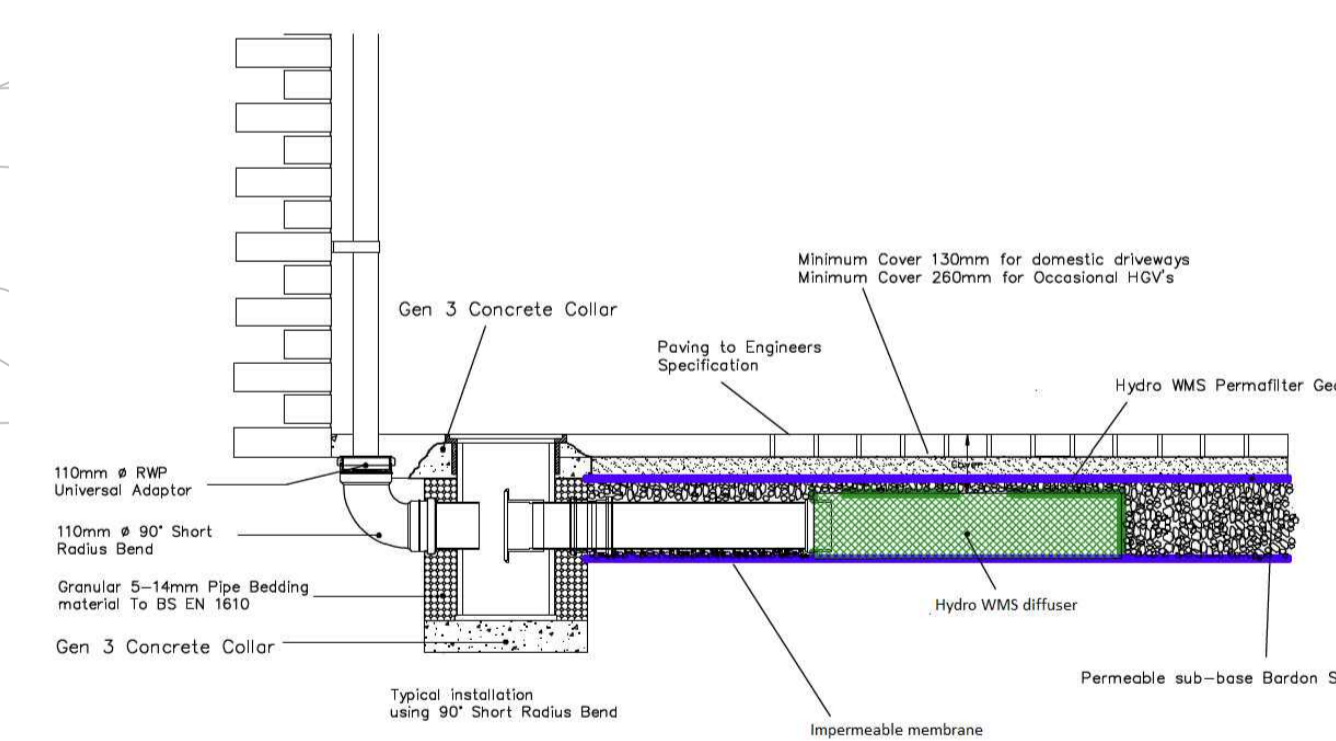
Typical section showing Inlet to Infiltration System
